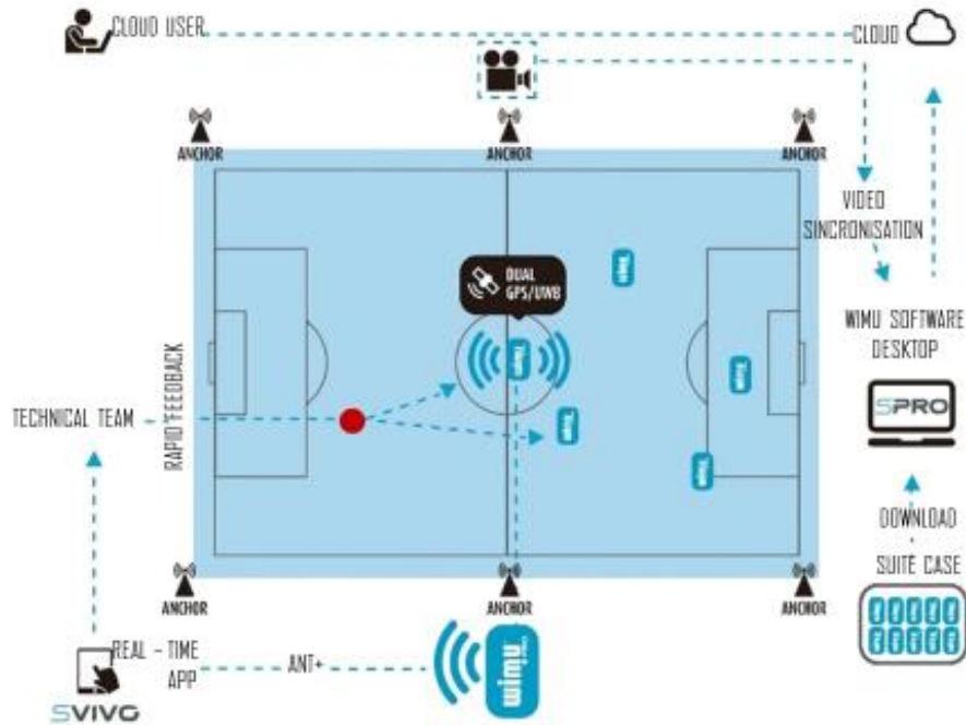
Figure 1 Graphical representation of the UWB data recording and analysis system.
